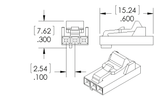
TE AmpModu MTE (Female)
